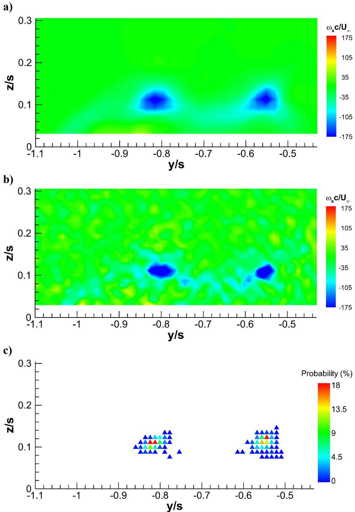
Figure 7. a) Time-averaged crossflow vorticity, b) instantaneous vorticity, and c) probability of instantaneous vortex locations in a crossflow plane over the double delta wing at \alpha = 12^\circ and x/c = 0.75 .
