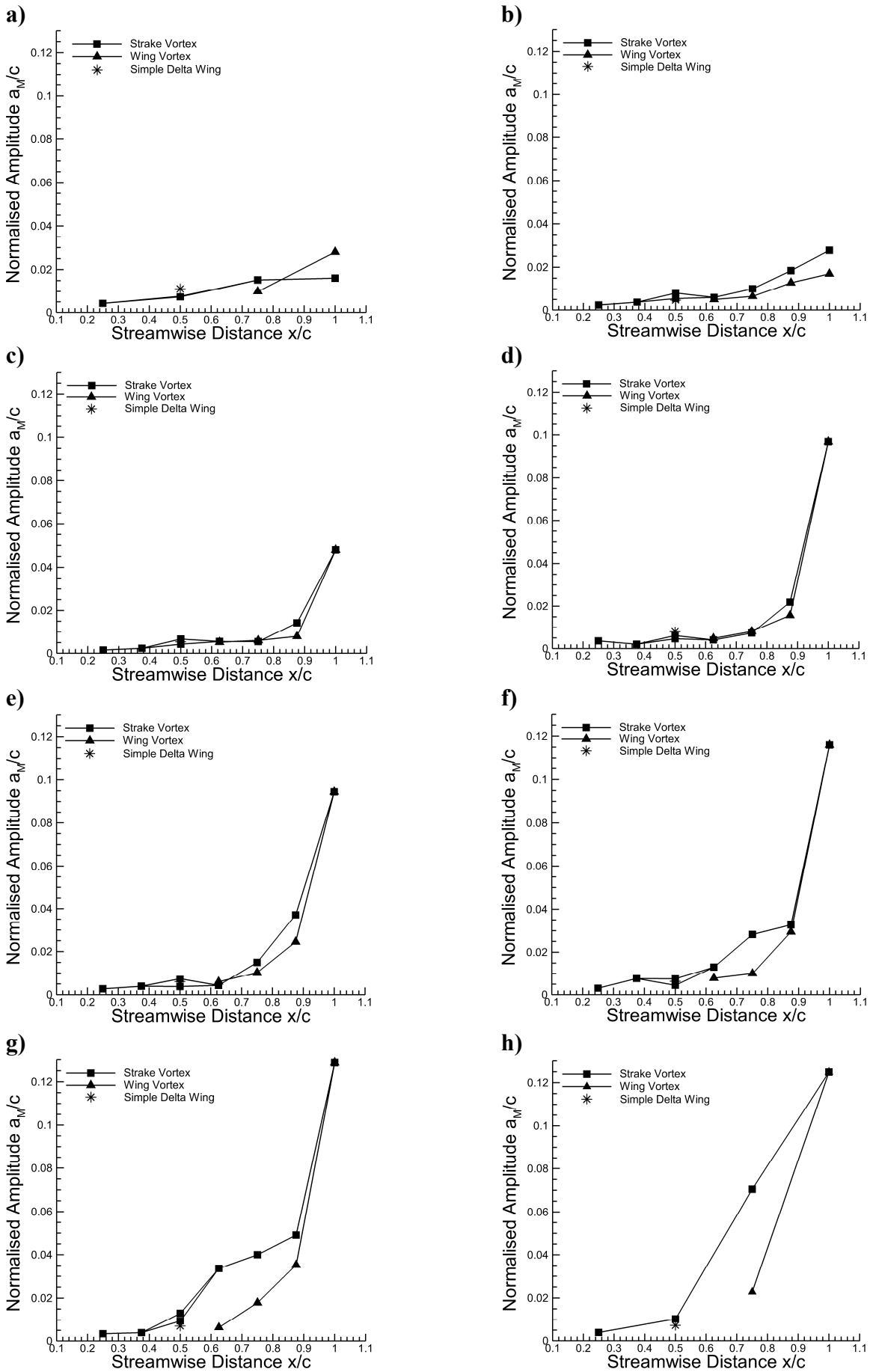
Figure 9. Variation of vortex meandering amplitude as a function of streamwise distance x/c for a) \alpha = 4^\circ ; b) \alpha = 8^\circ ; c) \alpha = 12^\circ ; d) \alpha = 16^\circ ; e) \alpha = 20^\circ ; f) \alpha = 24^\circ ; g) \alpha = 28^\circ ; h) \alpha = 32^\circ .
