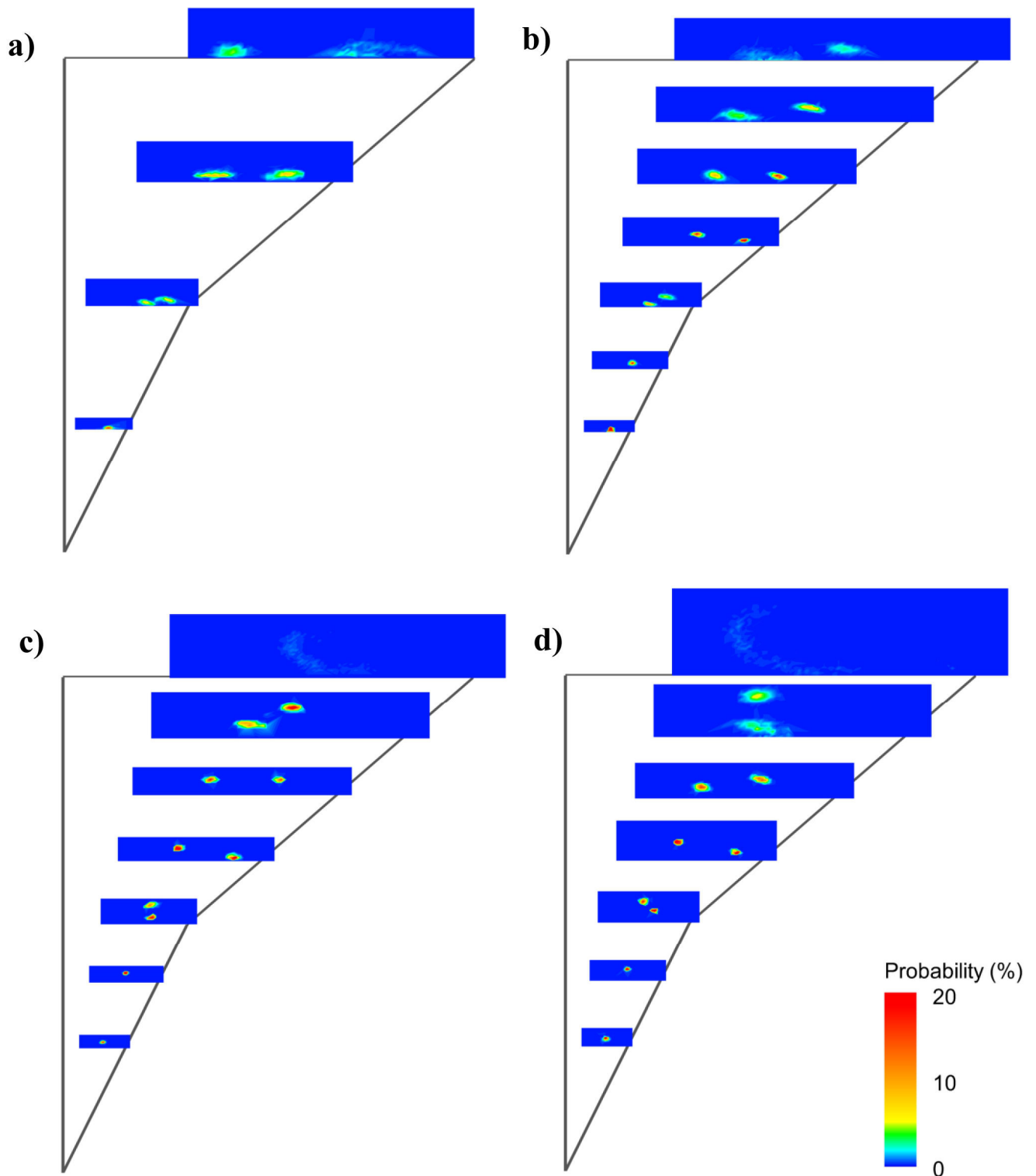
Figure 8. Probability of instantaneous vortex locations over the double delta wing at various chordwise locations for a) \alpha = 4^\circ ; b) \alpha = 8^\circ ; c) \alpha = 12^\circ ; d) \alpha = 16^\circ ; e) \alpha = 20^\circ ; f) \alpha = 24^\circ ; g) \alpha = 28^\circ ; h) \alpha = 32^\circ .
