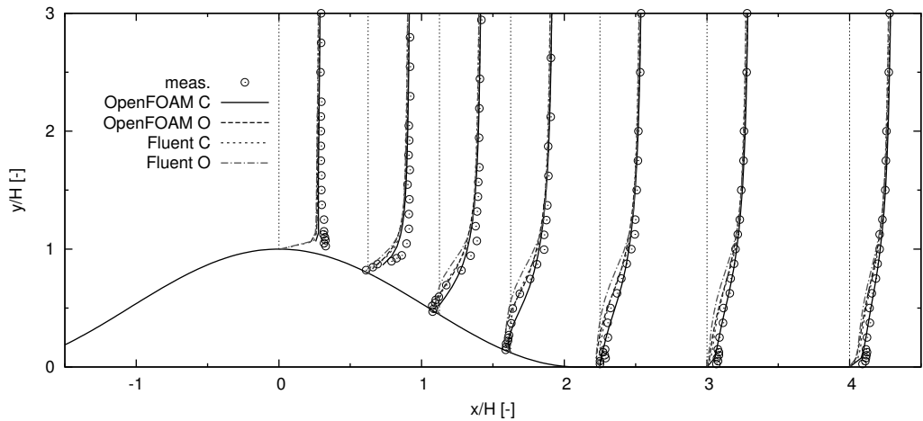
Streamwise velocity
