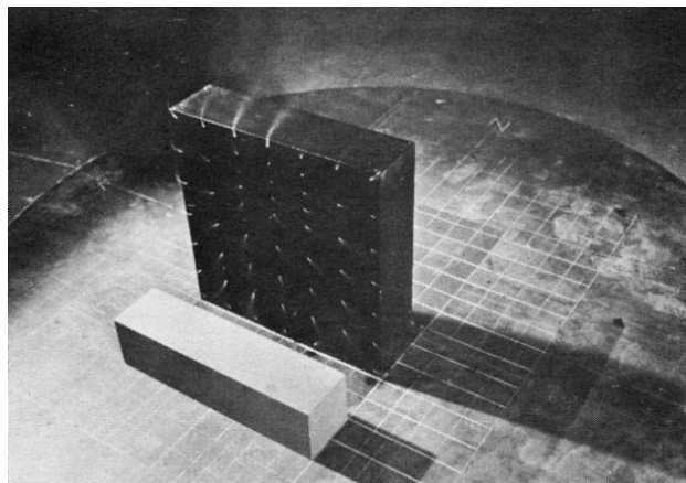
Flow around a slab block screened by a low building visualized by smoke in the wind tunnel
