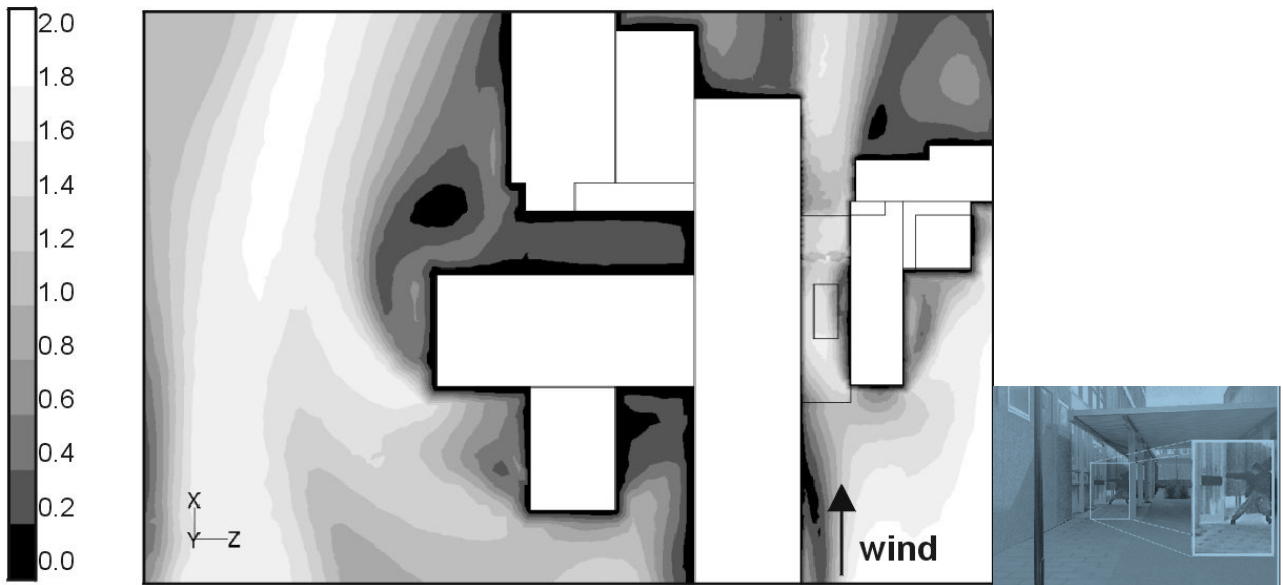
Contours of local amplification factor in a horizontal plane at 1.75m height above ground (pedestrian height). High wind amplification factors are found in the passage which are in clear contrast to the sheltered regions at the other side of the building.
