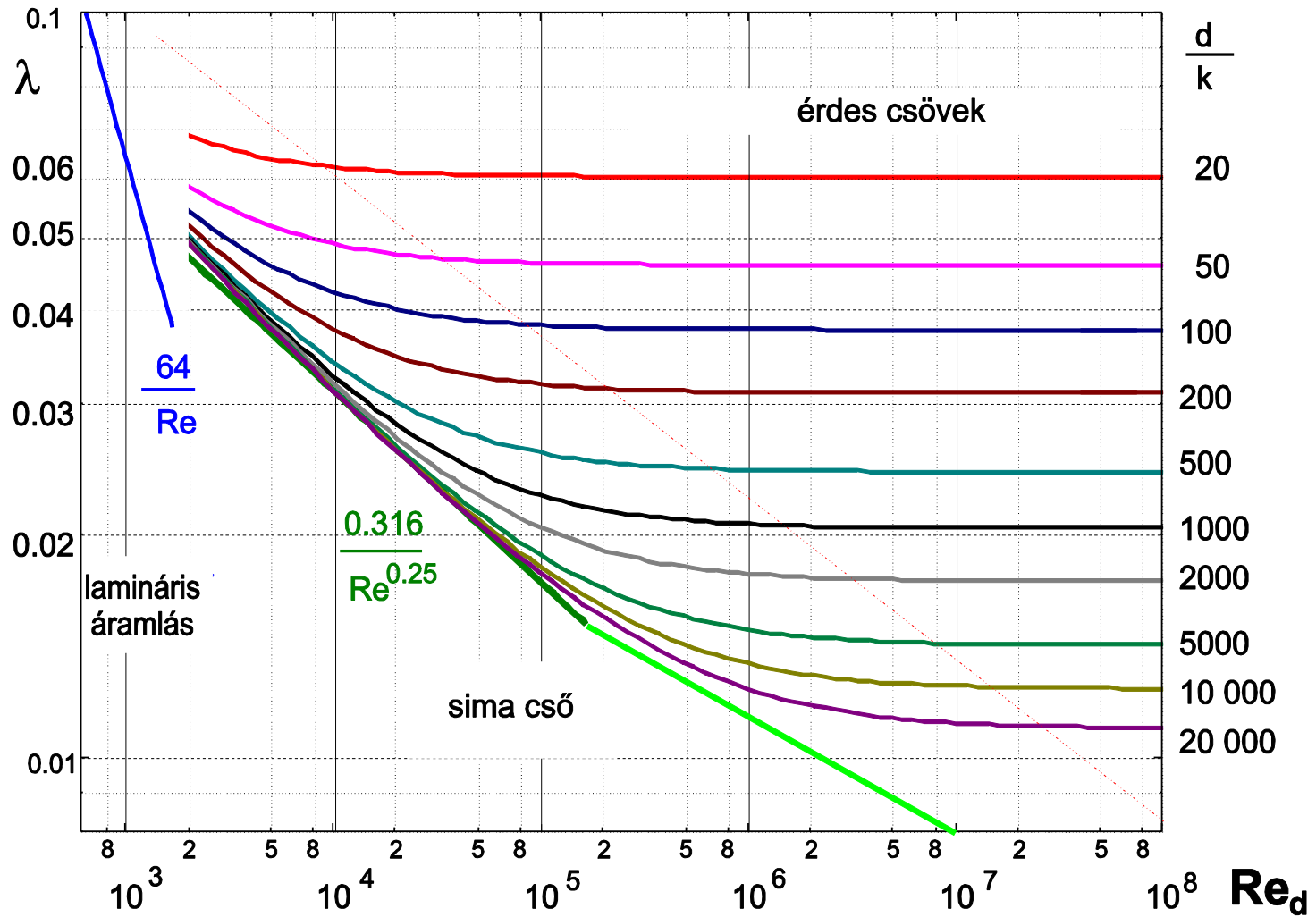
Moody-diagram
