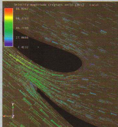
And velocity vectors through the slot gap show the flow accelerating under the flap
