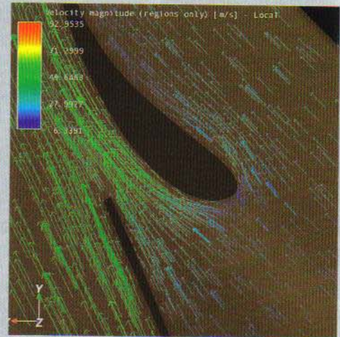
Figure 18 Underside view of the four-element plus slot configuration with velocity vectors
