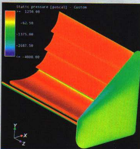
Figure 19 Static pressures on the upper surface of the four-element plus slot wing
