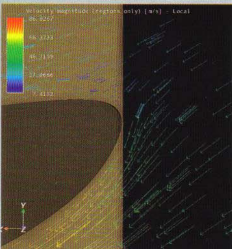
Velocity vectors show the stagnation point on the leading edge of the dual-element wing to be almost ideally located
