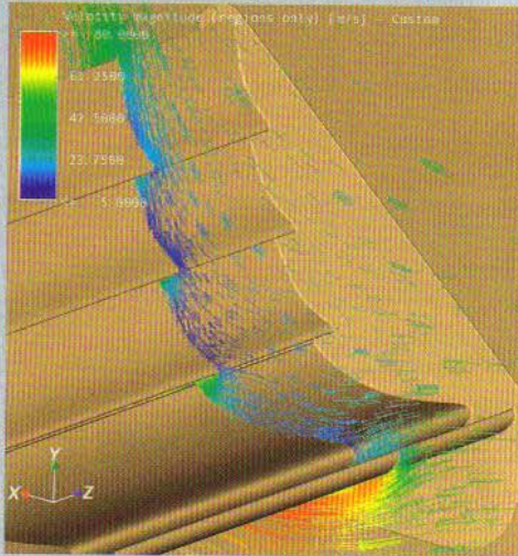
Figure 17 The four-element plus slot final configuration, with velocity vectors illustrating just how much the airflow is turned by this type of wing
