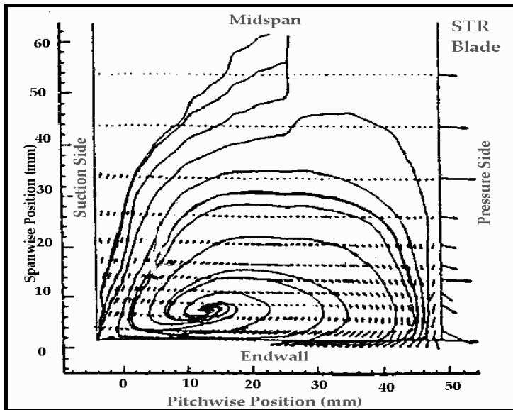
Fig. 3.4. Secondary vortex (passage vortex) detected in the vicinity of the annulus wall of a compressor cascade. Measurement data [13]
