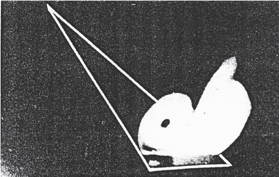
Fig. 6. Vortex formation behind Delta wing Aspect ratio=0.56, Reynolds number =132,000 \alpha = 35
