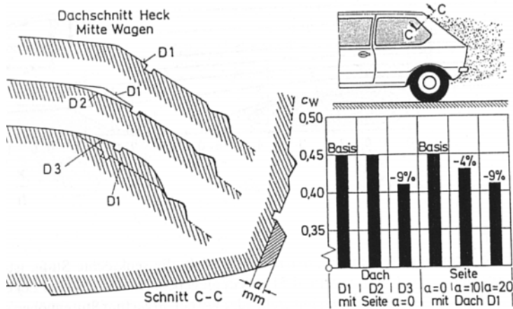
Practical realizations of tapering
